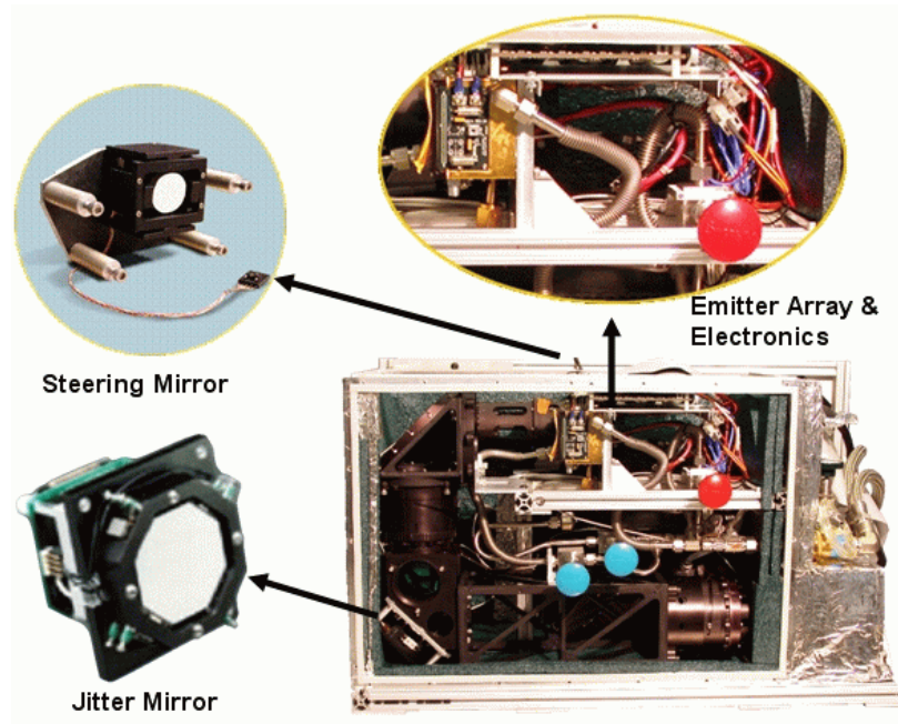
Figure 4: Subsystem Integration
