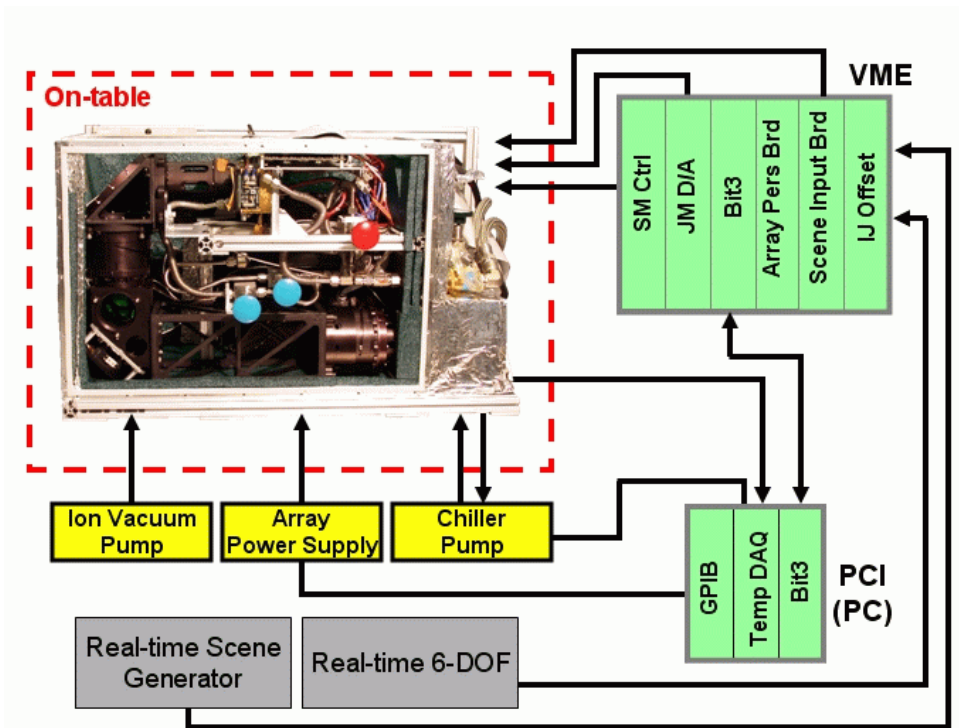
Figure 5: FMS IRSP Control Hardware
